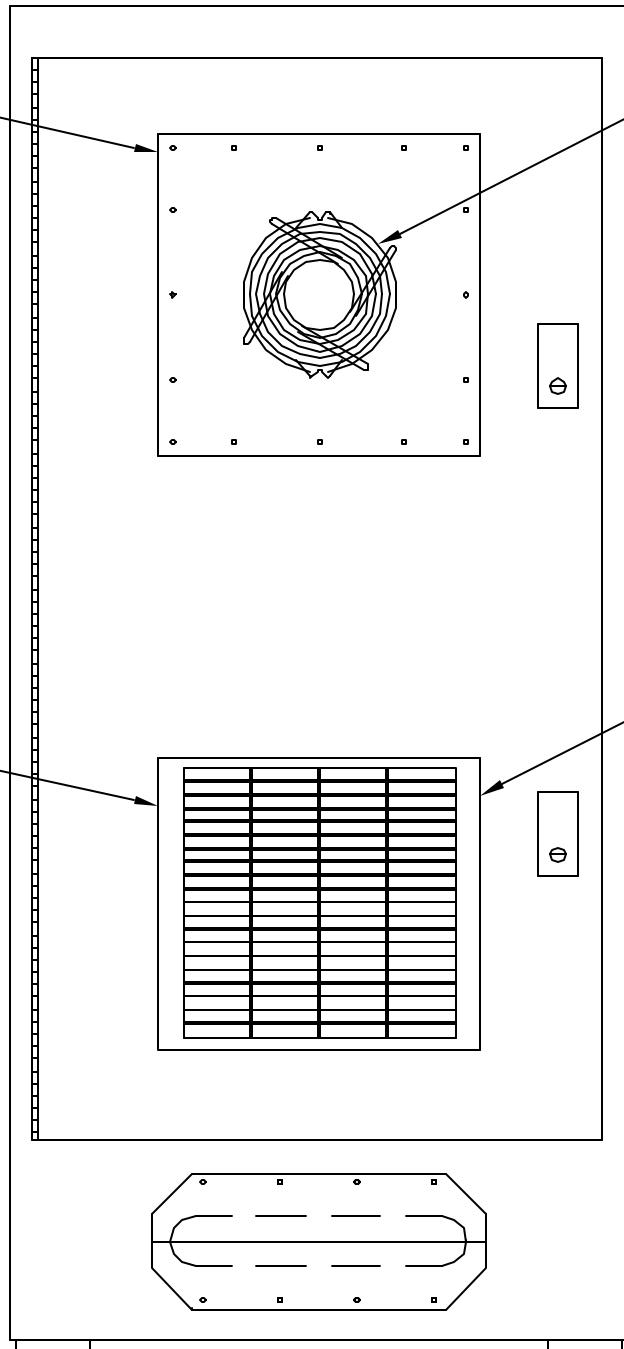
VIEW OF ENCLOSURE REAR DOOR SHOWN WITH VENTILATING FAN/FILTER
